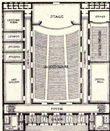
FIRST FLOOR PLAN PROPOSED FINE ARTS BUILDING FOR THE ASSOCIATED ARTS AND MUSICAL INTERESTS OF THE CITY OF PEORIA WARREN W DAY ARCHITECT
